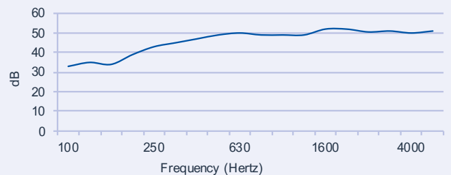
1/3 octave transmission loss Rw 50 door
