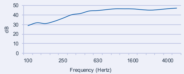
1/3 octave transmission loss Rw 50 door
