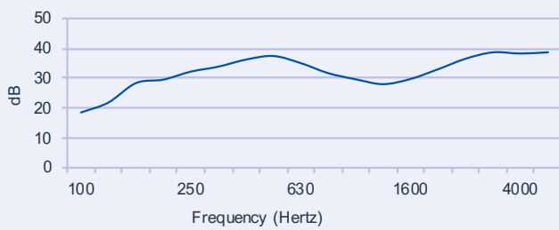
1/3 octave transmission loss Rw 47 door
