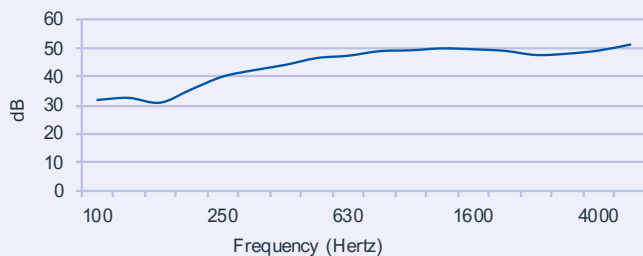
1/3 octave transmission loss Rw 47 door
